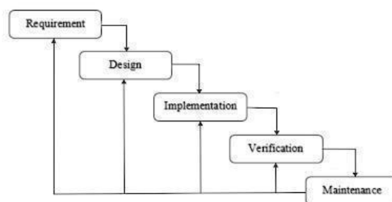
Gambar 1 Waterfall Model
