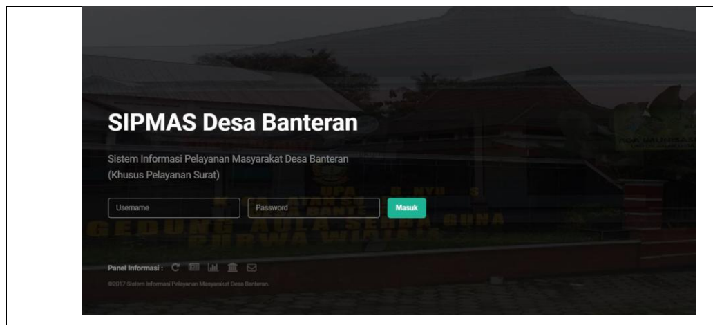
Gambar 2. Halaman Index
